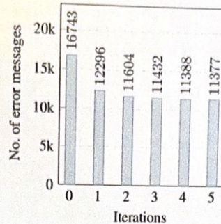
Figure 5: Number of error messages after each iteration on the raw dataset.
