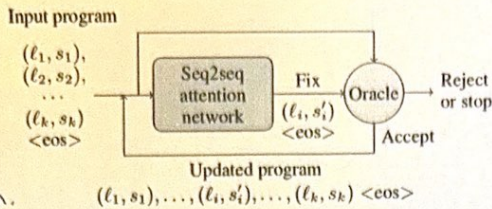
Figure 2: The iterative repair strategy of DeepFix.
