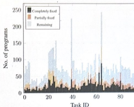
Figure 3: Task-wise reduction in erroneous programs for the raw dataset.
