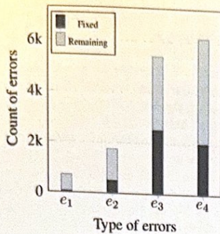
Figure 4: Top-4 types of error messages and their numbers before and after the fixes for the raw dataset.
